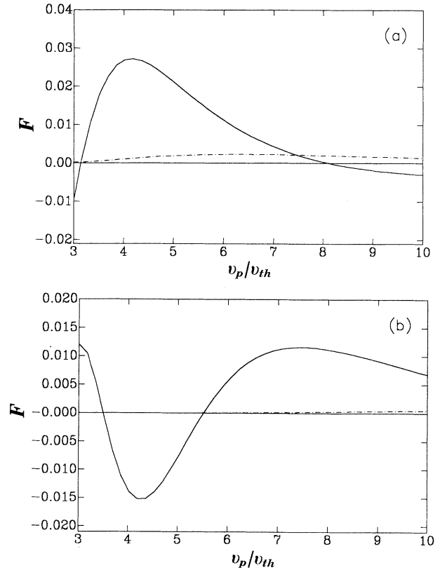
FIG. 1. Collective (solid line) and individual (dashed-dotted line) contributions to the mutual forces for \vartheta = 0^\circ given by Eqs. (7a) and (7c) as a function of v_p (in units of v_{th} ) for different values of l_b (in units of \lambda_D ): (a) l_b = 10 , (b) l_b = 20 . The plasma parameters are T = 20 \text{ eV} and n_0 = 10^{18} \text{ cm}^{-3} , while Z_{\text{eff}} = 10 for the projectiles.
