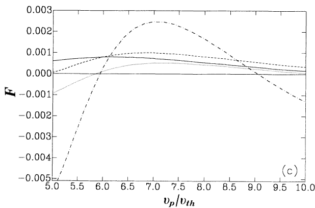
FIG. 2. The different components of the mutual forces, Eqs. (11), as a function of v_p for (a) l_b=10 , \vartheta=10^\circ ; (b) l_b=20 , \vartheta=10^\circ ; (c) l_b=20 , \vartheta=30^\circ . The plasma parameters are T=100 eV and n_0=10^{20} cm ^{-3} , and Z_{\text{eff}}=10 . Solid line F_{12,\parallel}^R ; dotted line, F_{12,\perp}^R ; dashed line, F_{12,\parallel}^{\text{NR}} ; dash-dotted line, F_{12,\perp}^{\text{NR}} . It can be noted that F_{12,\perp}^{\text{NR}} is, in modulus, always greater than the other components.
