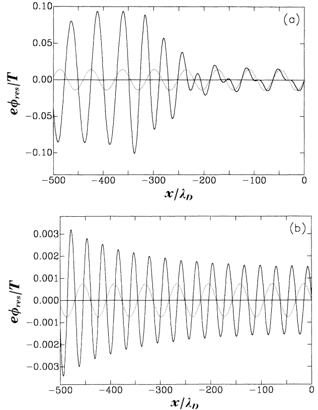
FIG. 9. Resonant contribution to the potential of an ion with v_p = 10 as a function of x for different values of \rho . (a) \rho = 40 , (b) \rho = 100 . Solid line, Eq. (A3); dotted line, Eq. (A6).
