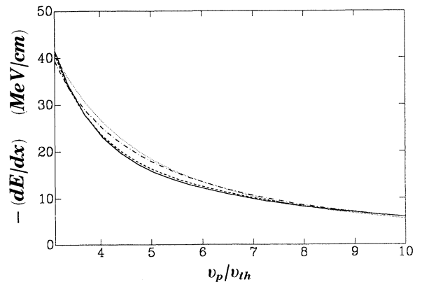
FIG. 4. Stopping power (in MeV/cm) of a two-ion correlated system with l_b = 10 as a function of v_p for different values of \vartheta . Solid line, \vartheta = 0^\circ ; dashed line, \vartheta = 10^\circ ; dash-dotted line, \vartheta = 25^\circ ; dotted line, single-particle approximation. Parameters as in Fig. 2.
