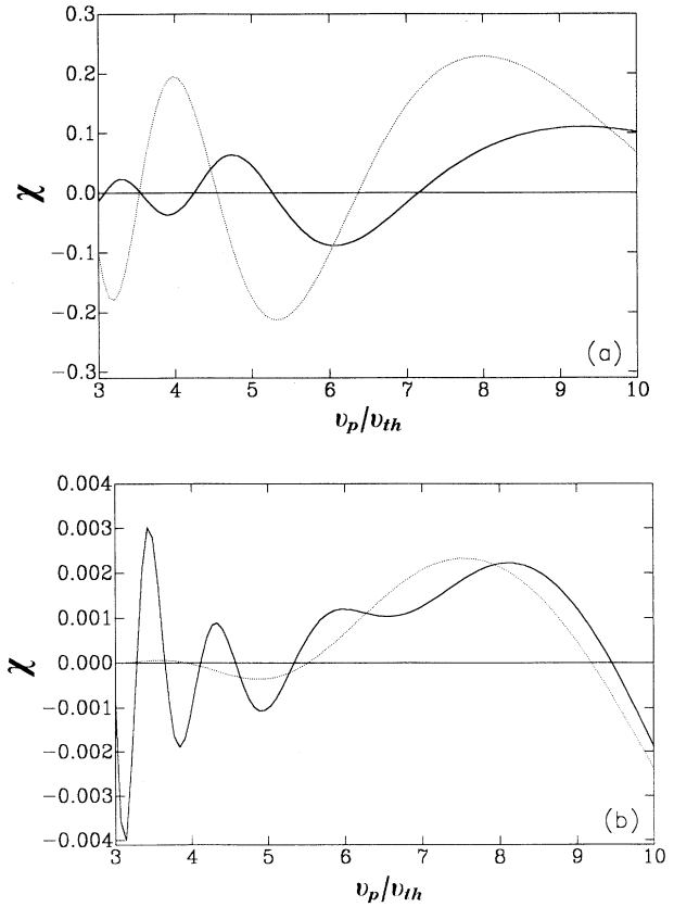
FIG. 6. Comparison between the \chi parameter within the two approximations X \approx -1/\xi^2 - 3/\xi^4 (solid line) and X \approx -1/\xi^2 (dotted line) as a function of v_p with l_b = 50 and with (a) \vartheta = 0^\circ , (b) \vartheta = 30^\circ . The plasma parameters are T = 10 eV and n_0 = 10^{18} \text{cm}^{-3} , with Z_{\text{eff}} = 10 for the projectiles.
