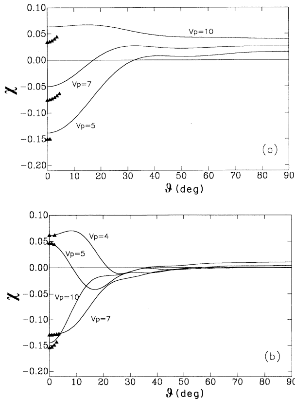
FIG. 5. The \chi parameter as a function of \vartheta for (a) l_b = 10 , (b) l_b = 20 , with the parameters as in Fig. 2. Solid line, \chi = \chi_{\text{coll}} ; \blacktriangle , \chi = \chi_{\text{coll}} + \chi_{\text{ind}} computed for \vartheta < 10^\circ .
