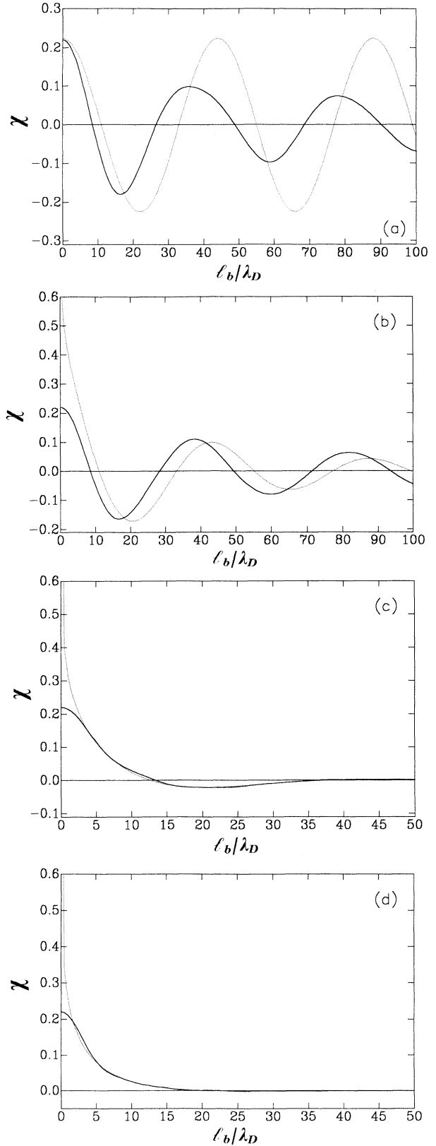
FIG. 7. Comparison between the \chi parameter within the two approximations, as in Fig. 6, as a function of l_b for v_p = 7 . (a) \vartheta = 0^\circ , (b) \vartheta = 5^\circ , (c) \vartheta = 30^\circ , (d) \vartheta = 60^\circ . The parameters are the same as in Fig. 6.
