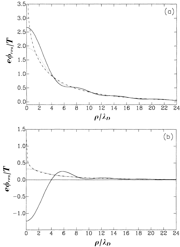
FIG. 8. Resonant contribution to the potential of an ion penetrating in a Maxwellian plasma with v_p = 10 as a function of \rho for different values of x . (a) x = 10 , (b) x = 30 . Solid line, Eq. (A3); dotted line, Eq. (A6), dashed-dotted line, Eq. (A8).
