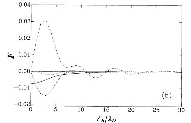
FIG. 3. The different components of the mutual forces, as in Fig. 2, as a function of l_b for v_p=7 and for (a) \vartheta=10^\circ , (b) \vartheta=60^\circ .
